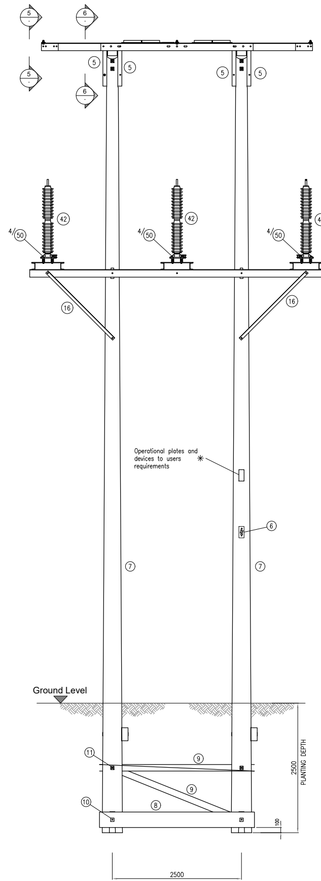
SECTION 1 Scale 1:35
