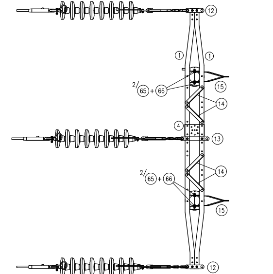
SECTION 4 Scale 1:35
