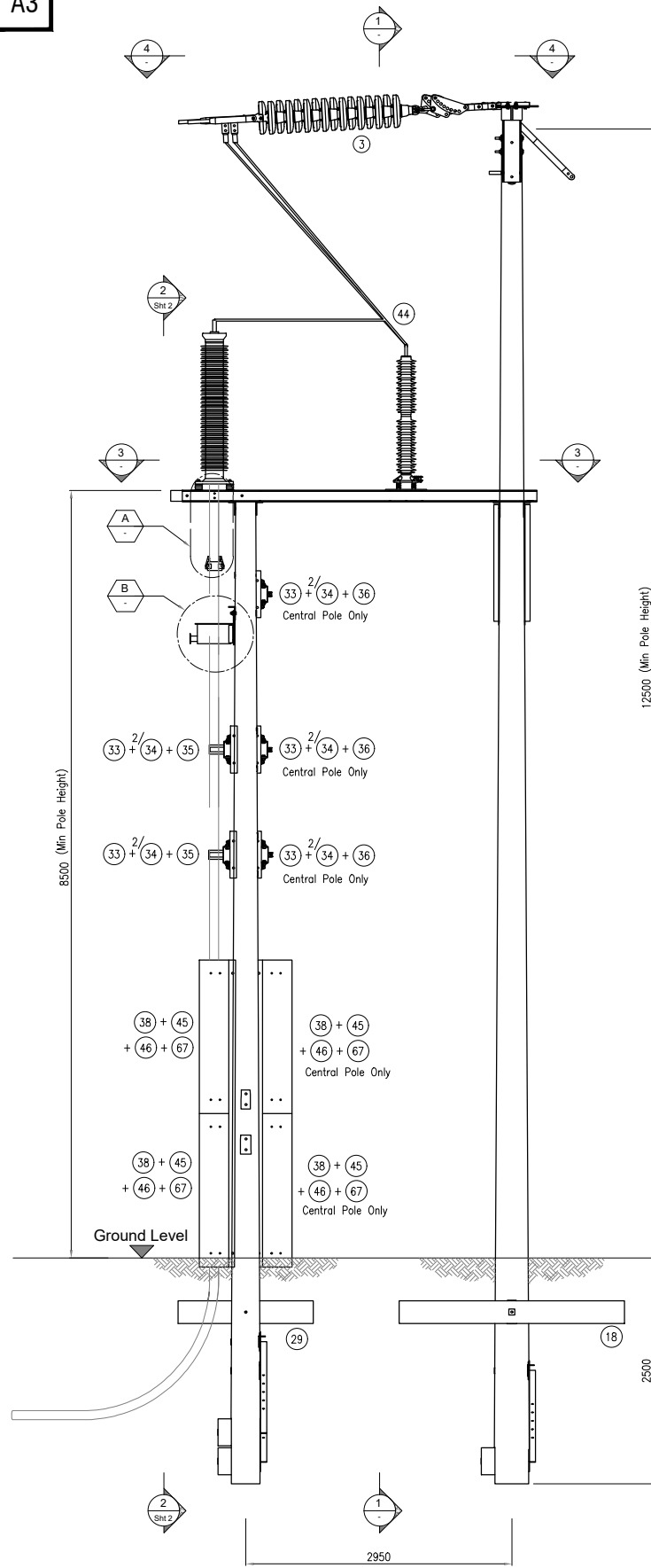
SIDE ELEVATION
